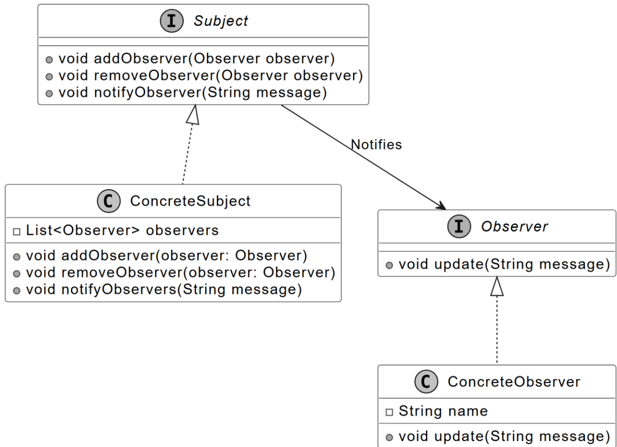
Observer design pattern class diagram
