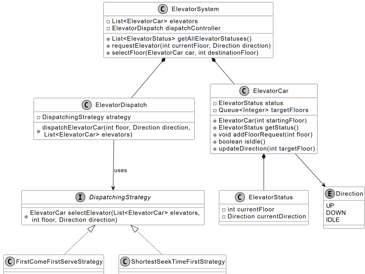
Class Diagram of Elevator System
