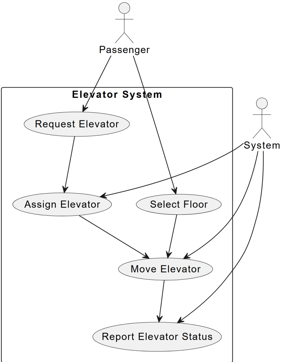
Use Case Diagram of Elevator Control System
